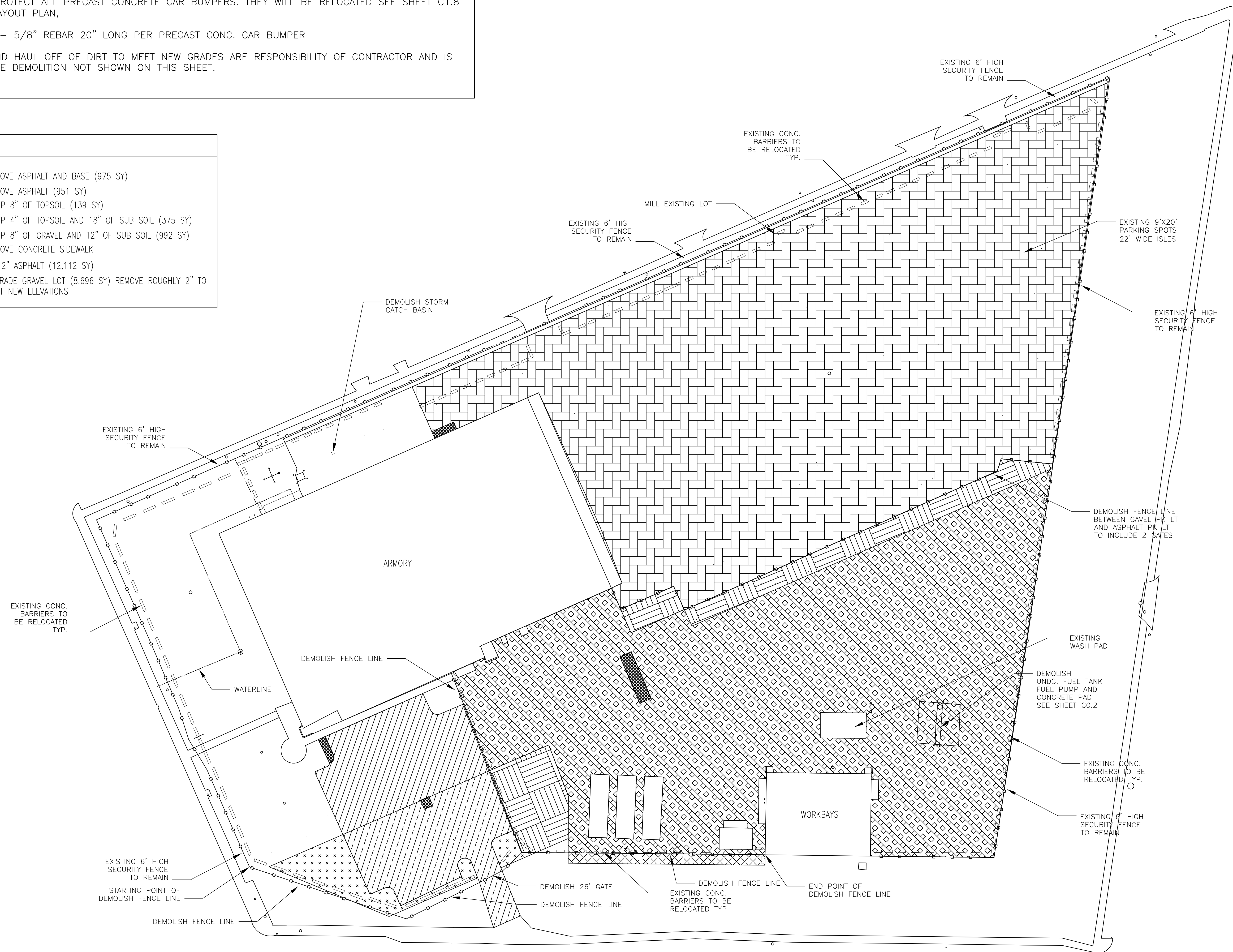
EXISTING SITE DEMO PLAN SCALE: 1" = 40'
